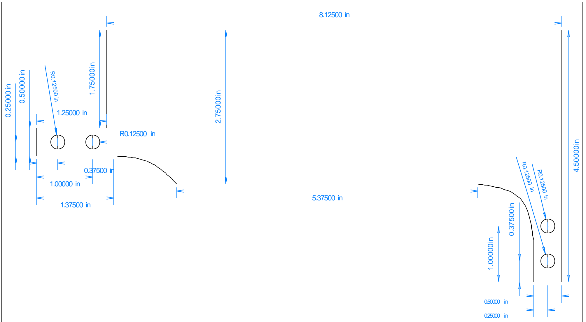
Monopoly Ramp Flap #2 - Design: Todd George - Date: 23-Oct-01
